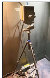
RADIANT VISION SYSTEM IMAGING PHOTOMETER
